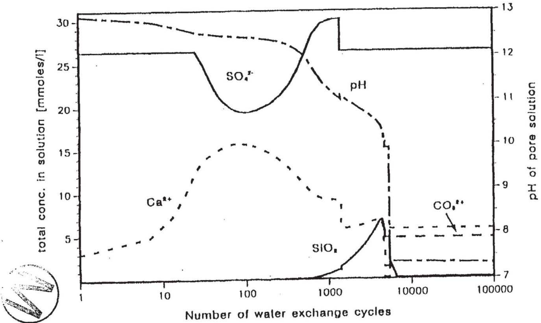
Figure c-3 Degradation of "HTS" in standard marl groundwater "MAR". After 6650 cycles calcite is the only solid phase present (T = 25 °C).
