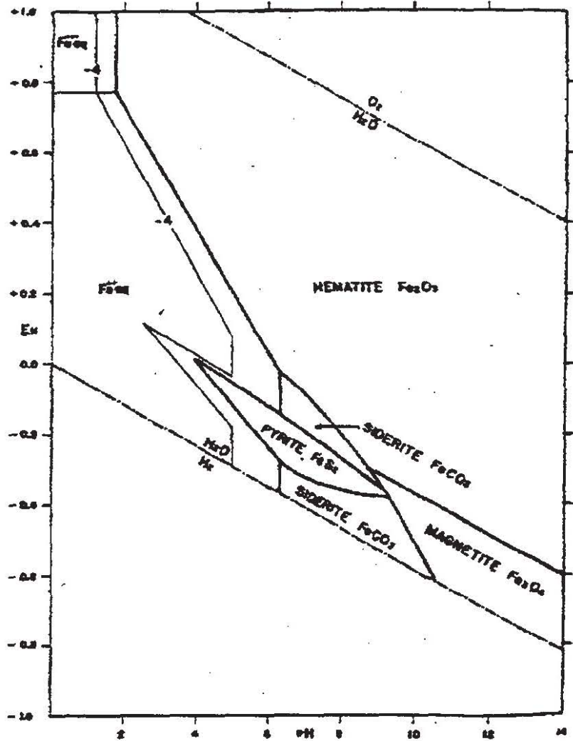
FIG B-3. Stability relations of iron oxides, sulfides, and carbonates in water at 25 °C and 1 atmosphere total pressure. Total dissolved sulfur = 10 -6 . Total dissolved carbonate = 10 -6 . Note elimination of Fe 3+ field by FeCO 3 under strongly reducing conditions, and remarkable stability of pyrite in presence of small amount dissolved sulfur.
